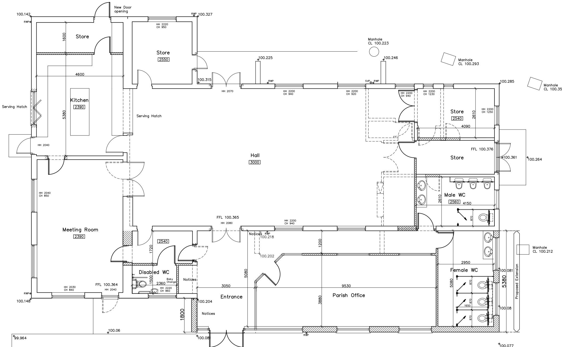
Ground Floor Plan scale 1:50 @ A1 (1:100 @ A3)
